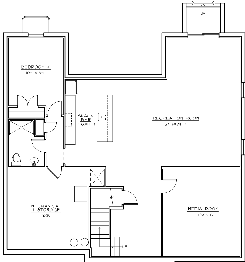
BASEMENT PLAN
